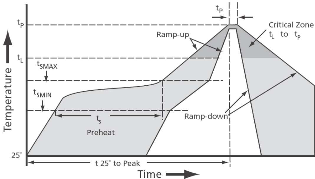
Figure 7. JEDEC reflow profiles for Sn-Pb AND Pb-free assemblies
